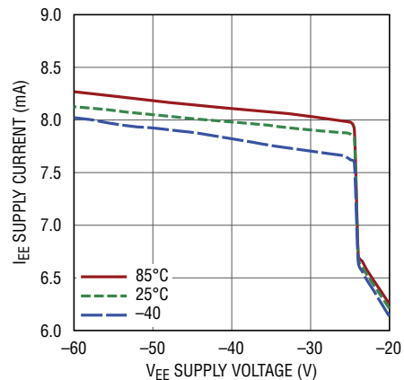
VEE Supply Current vs Voltage
