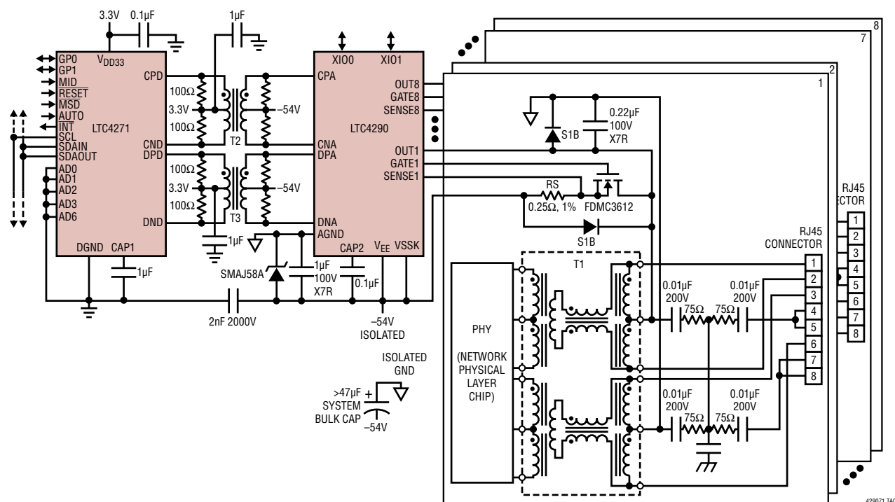
Complete 8-Port PSE
