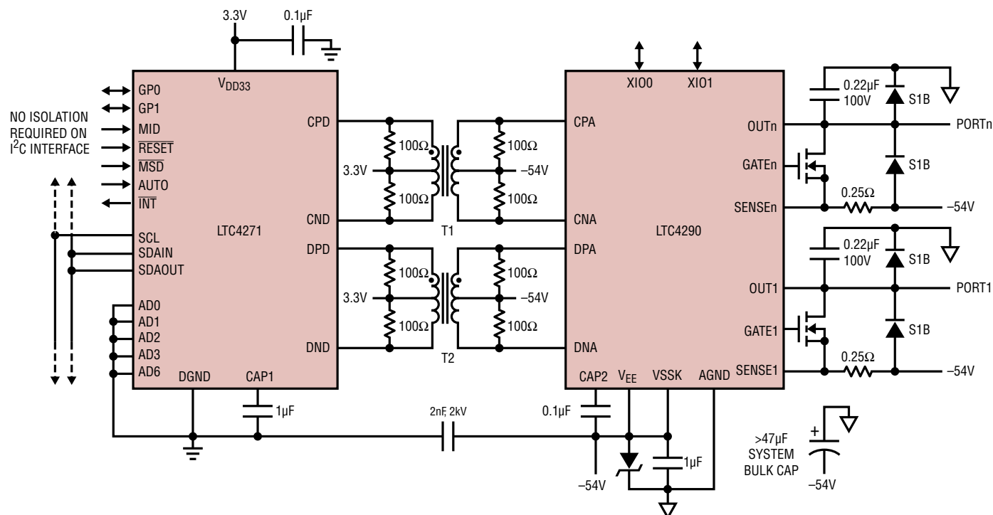
Figure 15. LTC4290/LTC4271 Proprietary Isolation
