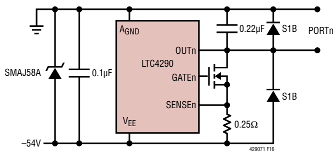
Figure 16. LTC4290 Discharge Protection
