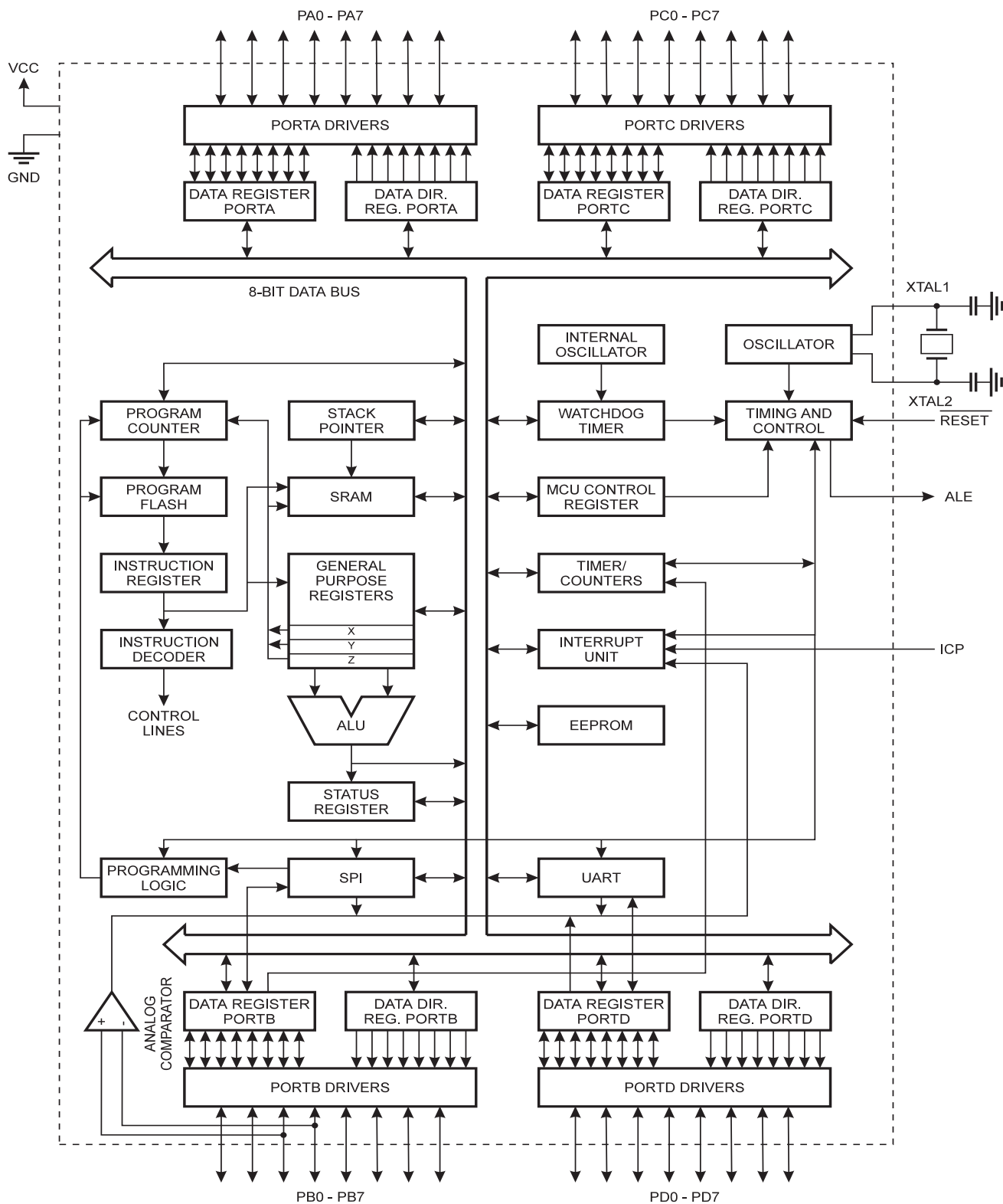
Figure 1. The AT90S4414 Block Diagram
