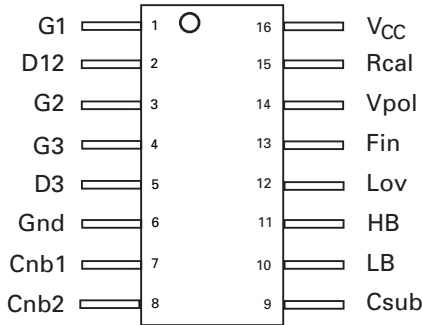
QSOP16
