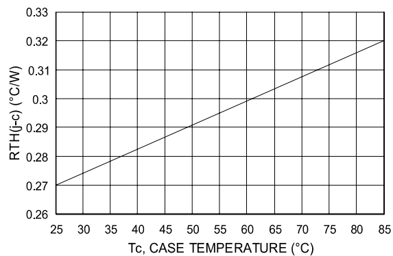
Figure 6: Maximum thermal resistance vs. case temperature
