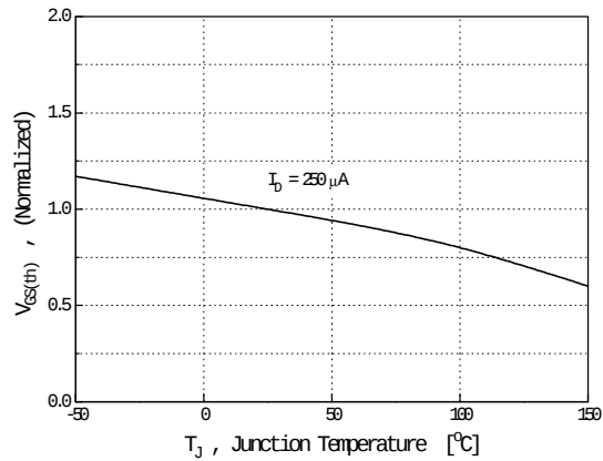
Fig 10. Threshold Voltage
