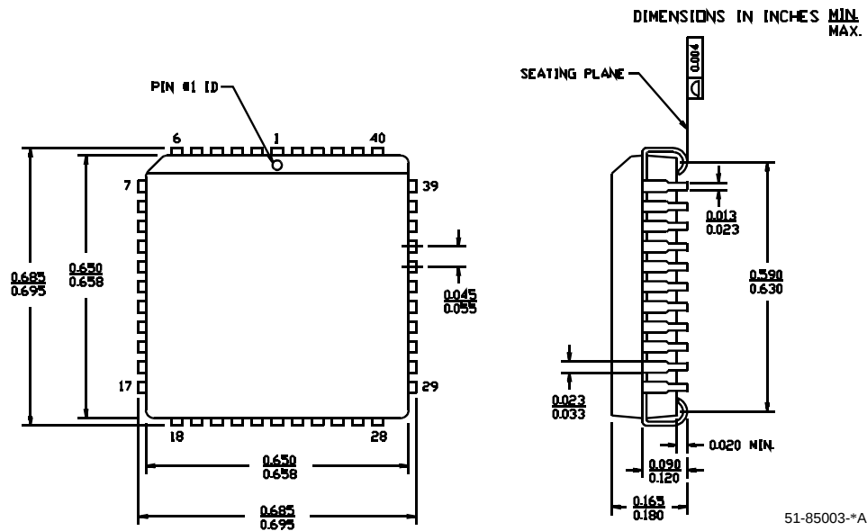
44-Lead Lead(Pb)-Free Plastic Ledged Chip Carrier J67
