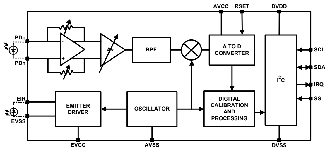
FIGURE 2. BLOCK DIAGRAM
