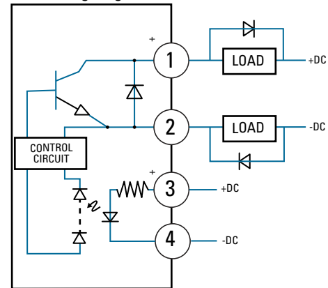
Wiring Diagram (4)
