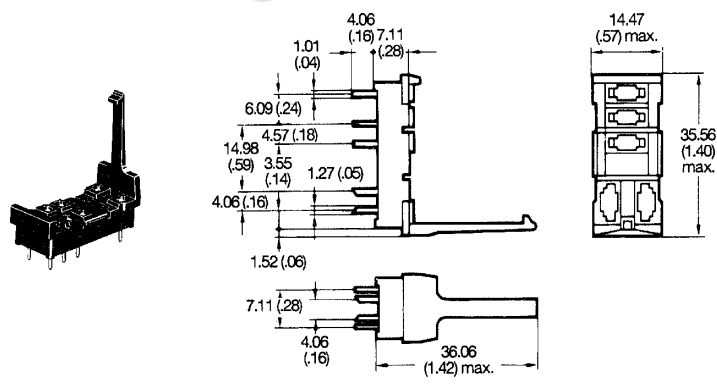
Terminal arrangement
