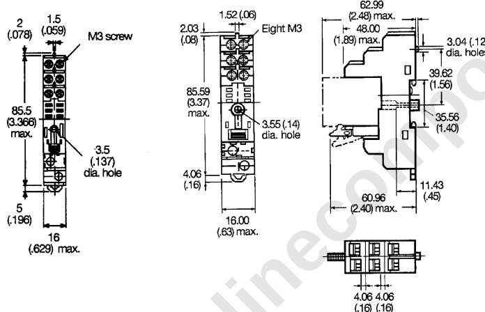
Terminal arrangement
