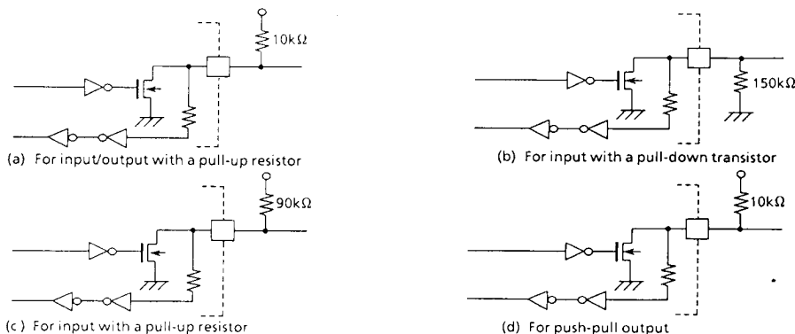
Figure 3. Example of external circuitry
