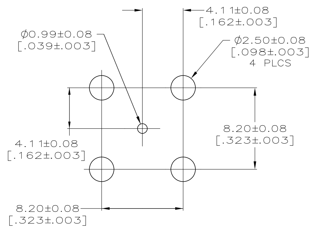
PCB CONFIGURATION
