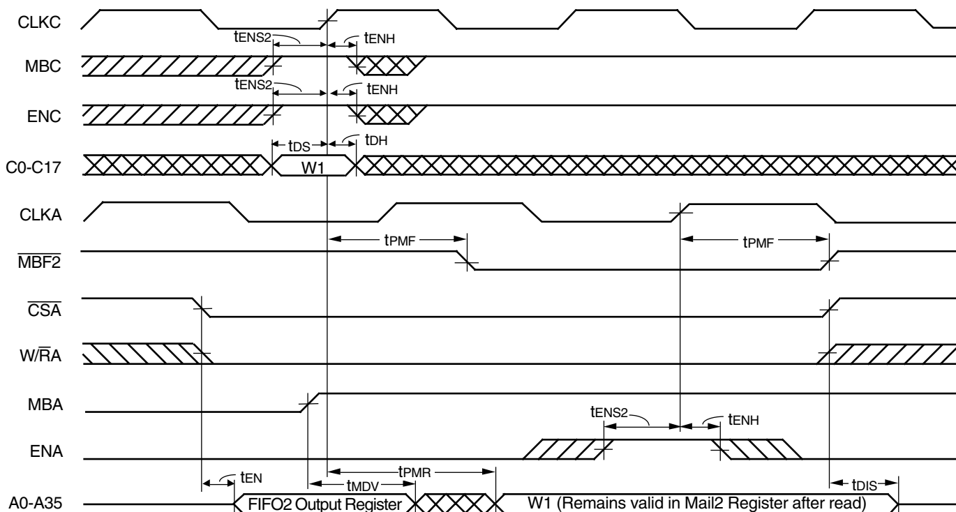
Figure 28. Timing for Mail1 Register and MBF1 Flag (IDT Standard and FWFT Modes)
