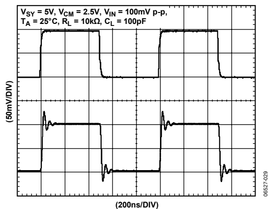
Figure 29. 5 V Small Signal Transient Response
