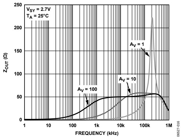
Figure 16. Z_{OUT} vs. Frequency
