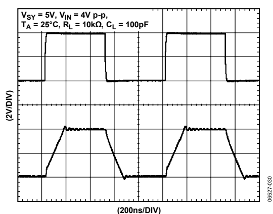
Figure 30. 5 V Large Signal Transient Response
