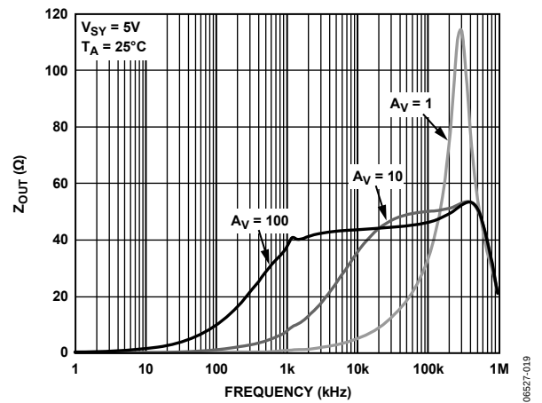
Figure 19. Z_{OUT} vs. Frequency
