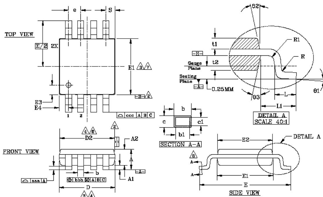
Figure 8. MSOP-8 Package
