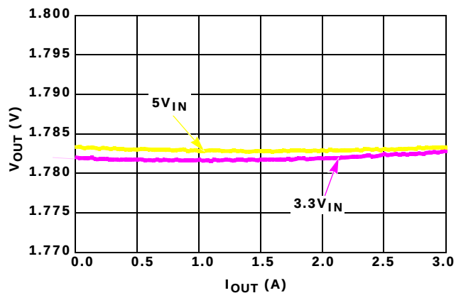
FIGURE 8. LOAD REGULATION, V_{OUT} = 1.8\text{V} , T_A = +25^\circ\text{C}
