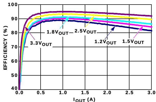
FIGURE 4. EFFICIENCY, T_A = +25^\circ\text{C} , V_{IN} = 5\text{V}
