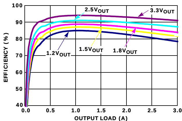
FIGURE 33. EFFICIENCY vs LOAD, 1MHz 5VIN, DUAL CH1 +25°C
