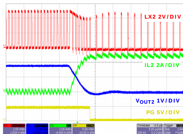
FIGURE 30. OUTPUT SHORT CIRCUIT CHANNEL 2
