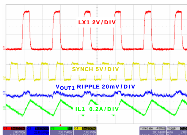
FIGURE 24. CHANNEL 1 STEADY STATE OPERATION AT NO LOAD WITH FREQUENCY = 6MHz
