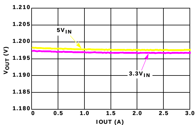
FIGURE 6. LOAD REGULATION, V_{OUT} = 1.2\text{V} , T_A = +25^\circ\text{C}
