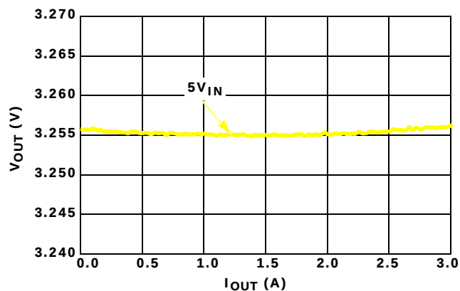
FIGURE 10. LOAD REGULATION, V_{OUT} = 3.3\text{V} T_A = +25^\circ\text{C}
