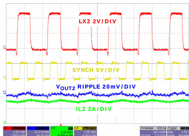
FIGURE 27. CHANNEL 2 STEADY STATE OPERATION AT FULL LOAD WITH FREQUENCY = 6 MHz
