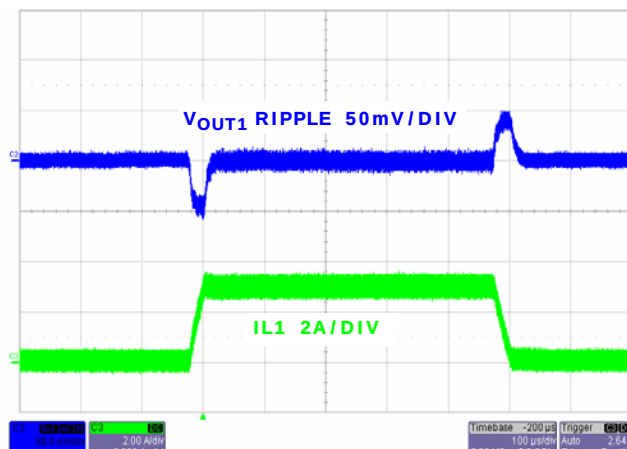
FIGURE 16. LOAD TRANSIENT CHANNEL 1 (PWM)
