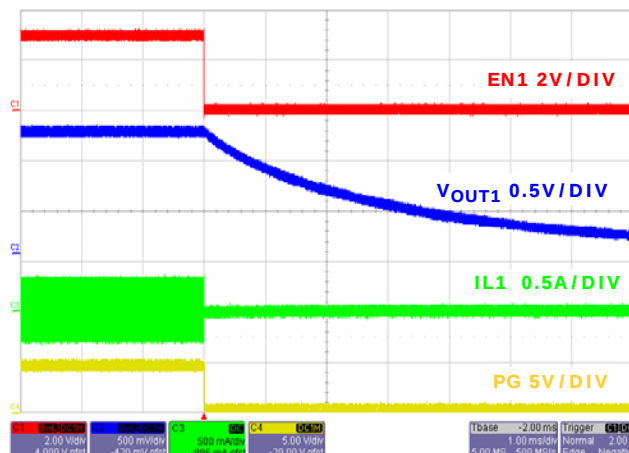
FIGURE 22. SOFT-DISCHARGE SHUTDOWN CHANNEL 1
