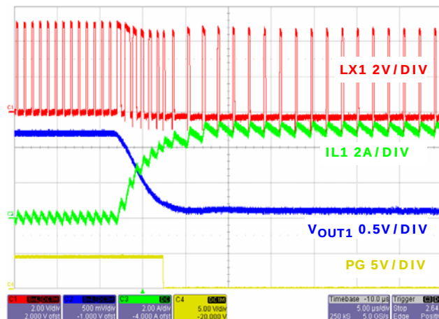
FIGURE 28. OUTPUT SHORT CIRCUIT CHANNEL 1
