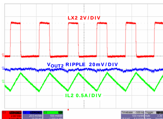
FIGURE 12. STEADY STATE OPERATION AT NO LOAD CHANNEL 2 (PWM)
