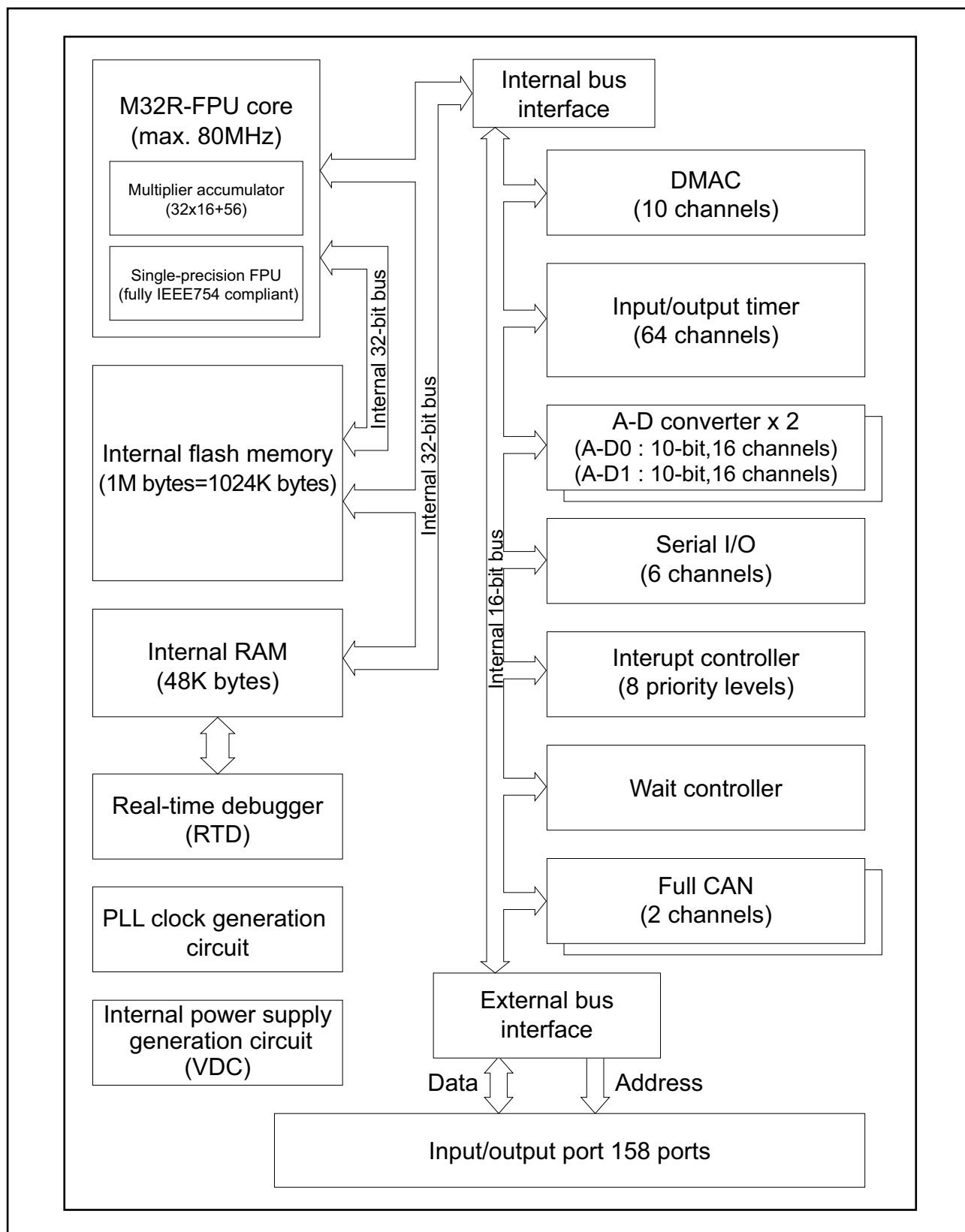
Figure 2. Block diagram
