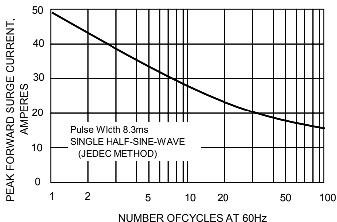
FIG.2-MXIMUM NON-REPETITIVE SURGE CURRENT
