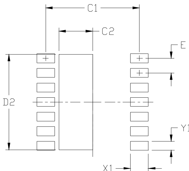
Figure 52. 14-Pin LGA with Thermal Pad Land Pattern
