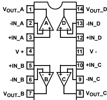
ISL28417 (14 LD SOIC, TSSOP) TOP VIEW
