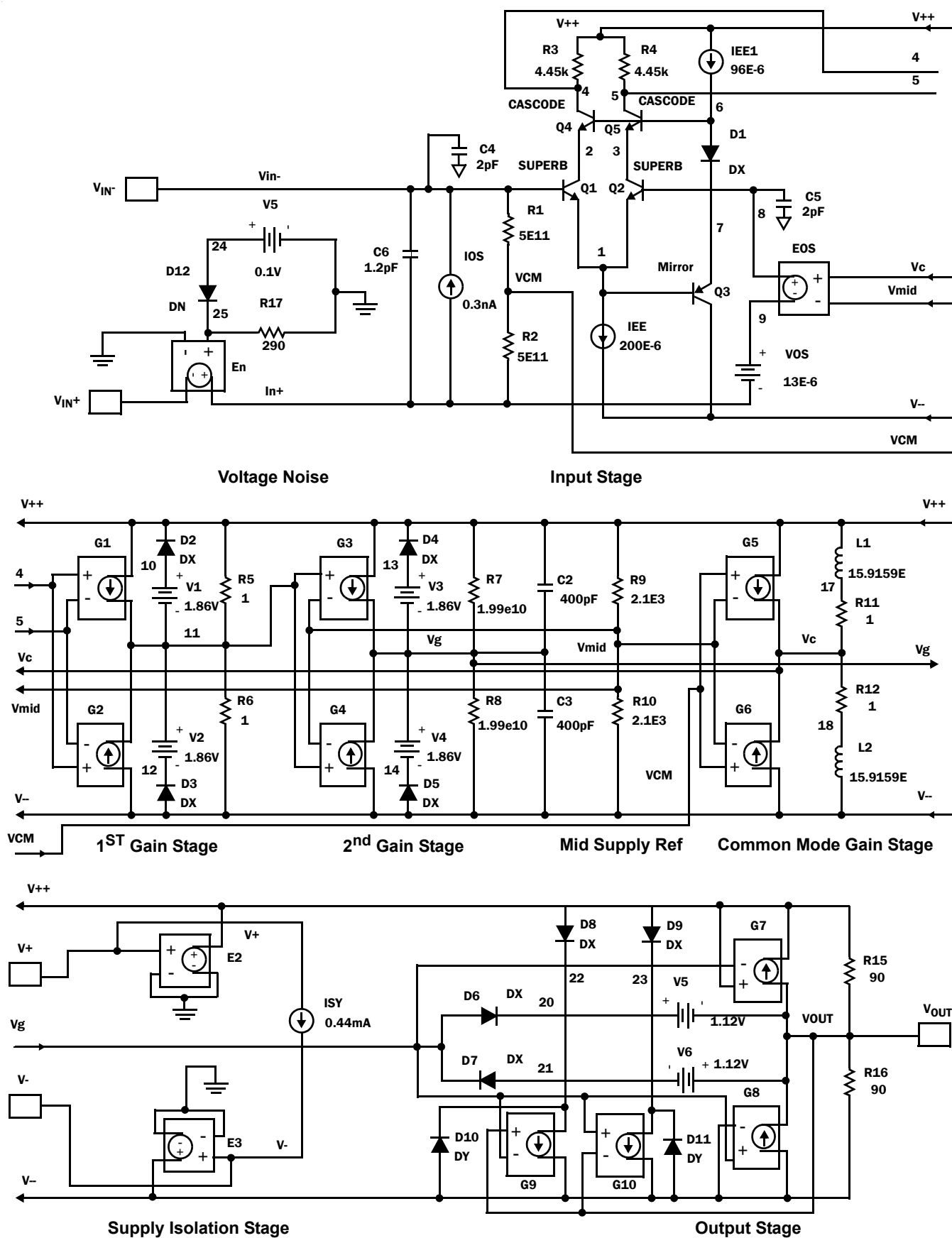
FIGURE 56. SPICE SCHEMATIC
