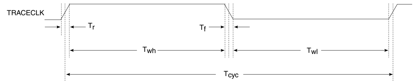
Figure 5. TRACE_CLKOUT specifications
