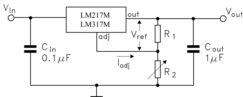
Figure 3. Test circuit
