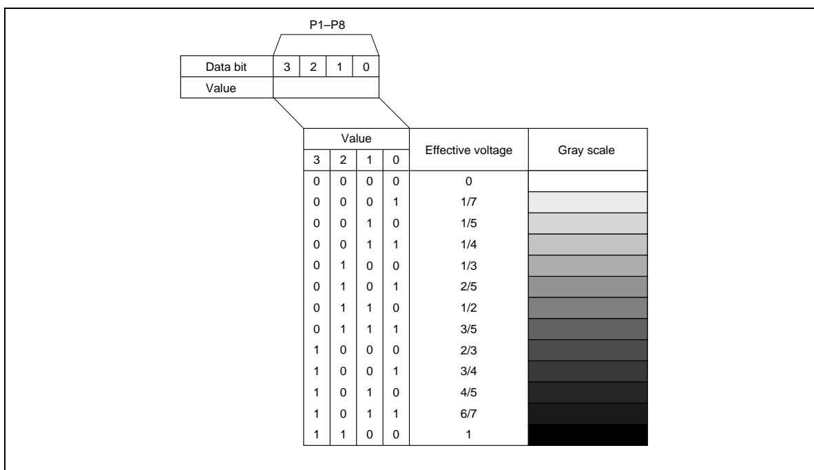
Figure 30 Palette Registers
