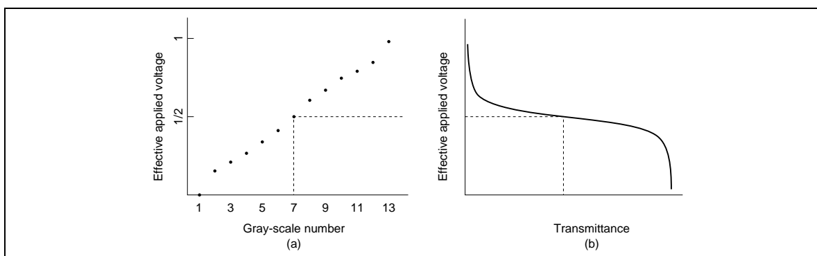
Figure 12 Relationships between Gray Scale, Transmittance, and Effective Applied Voltage
