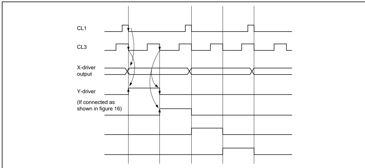
Figure 15 Relationship between CL1 and CL3 in Modes 1, 2, 4, 6, 7, and 8
