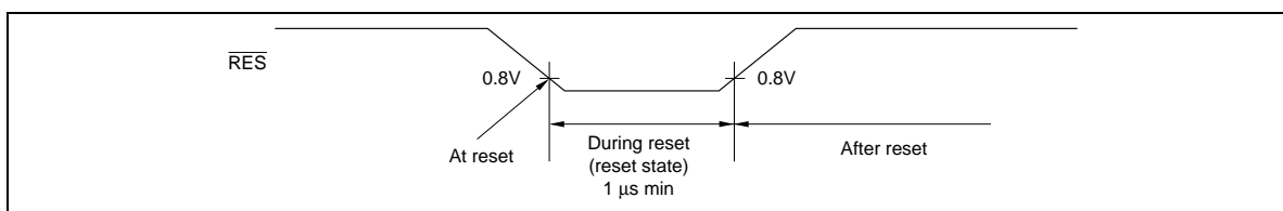
Figure 31 Reset Definition
