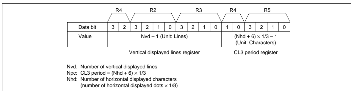
Figure 22 Vertical Displayed Lines Register and CL3 Period Register
