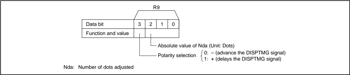
Figure 26 Fine Adjust Register
