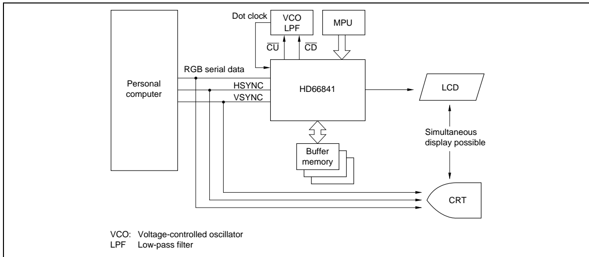
Figure 2 System Block Diagram (with MPU Programming Method and DOTCLK Generated Internally)
