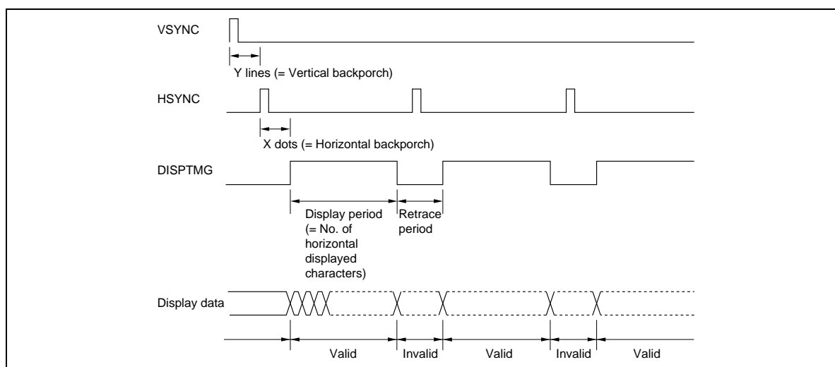
Figure 10 Relation between HSYNC, VSYNC, DISPTMG, and Display Data
