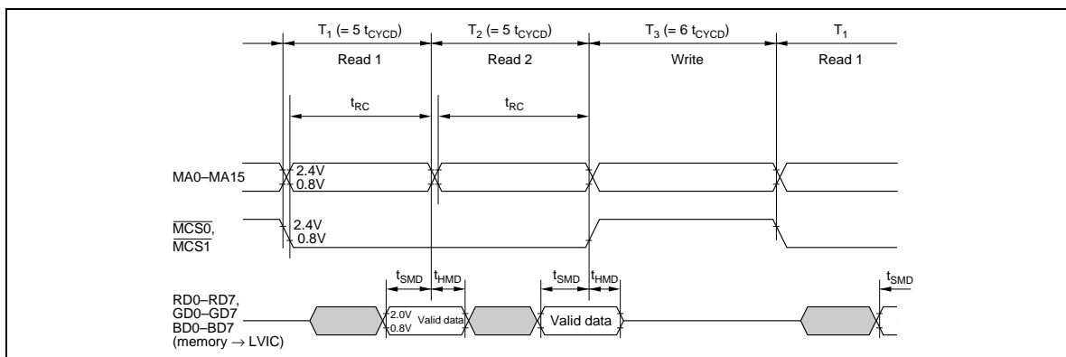
Figure 34 Buffer Memory Interface (RAM Read Timing)
