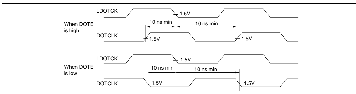
Figure 9 Relationships between DOTE and LDOTCK, DOTCLK
