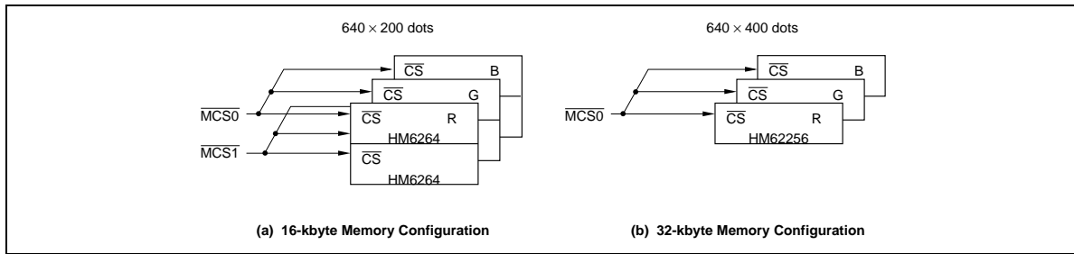
Figure 5 Screen Size and Memories Configuration
