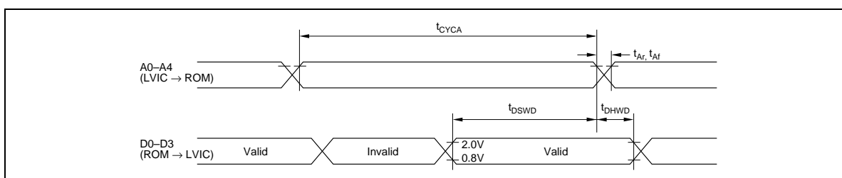
Figure 41 ROM Interface
