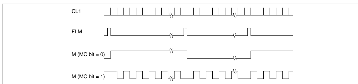
Figure 37 CL1, FLM, and M (Expanded Detail of Figure 34)
