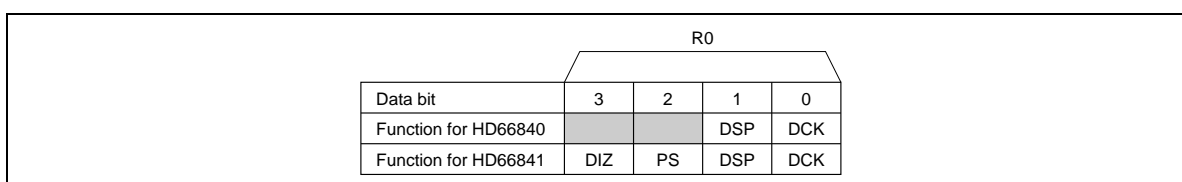
Figure 19 Control Register 1
