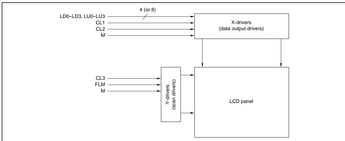
Figure 16 Connection for Double-Height Display
