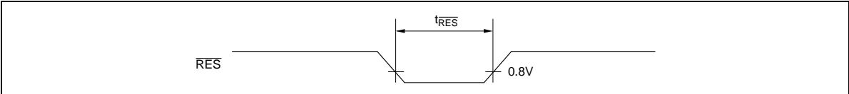
Figure 43 Reset Input
