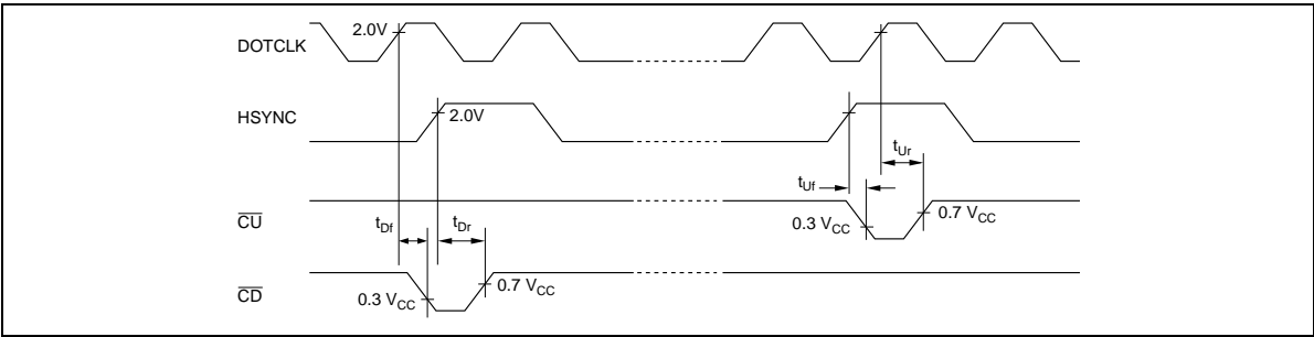
Figure 42 PLL Interface
