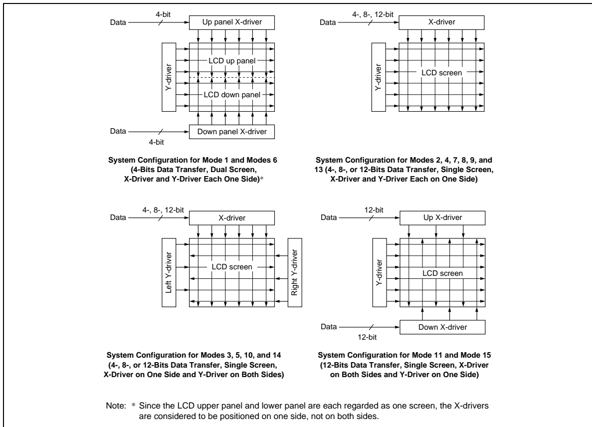
Figure 7 System Configurations by Mode
