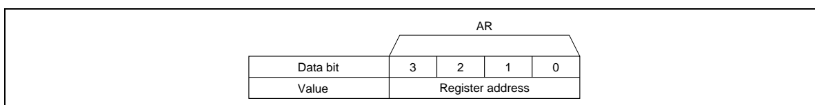
Figure 18 Address Register
