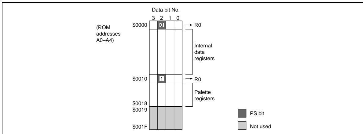
Figure 20 PS Bit Functions in ROM Programming Method
