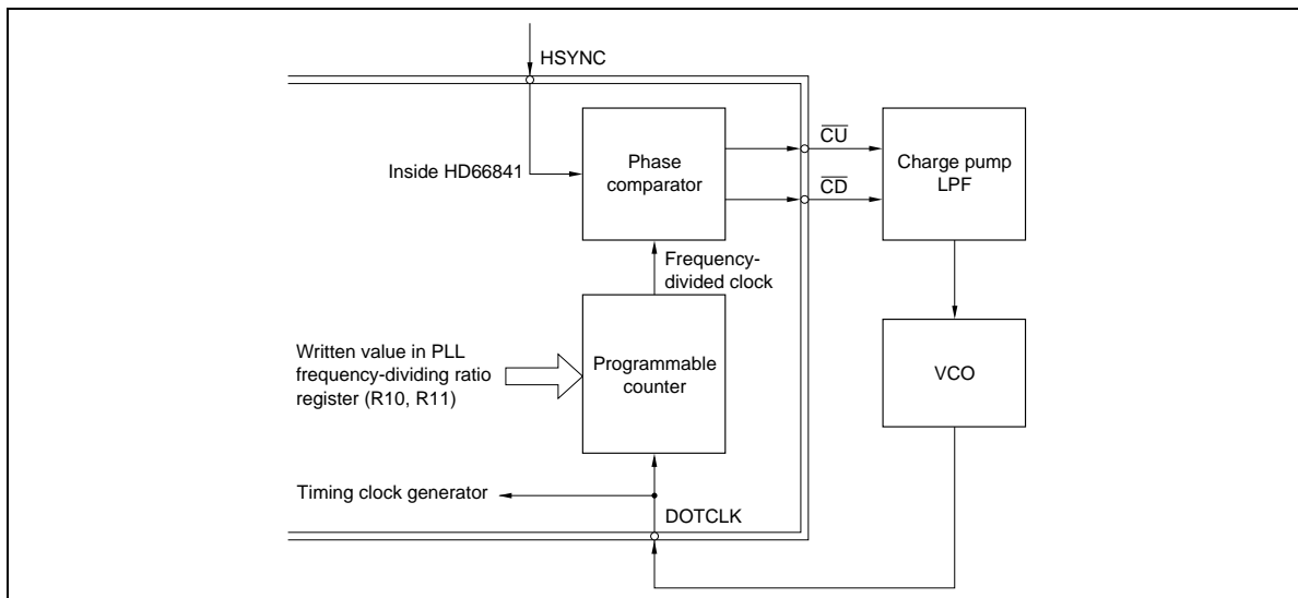
Figure 11 PLL Circuit Block Diagram
