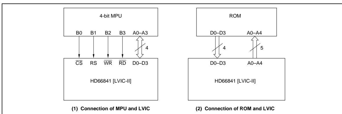
Figure 3 Connection of MPU or ROM and HD66841
