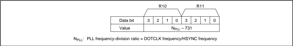
Figure 27 PLL Frequency-Division Ratio Register
