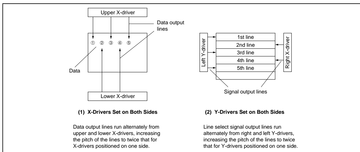
Figure 8 X- and Y-Drivers Set on Both Sides
