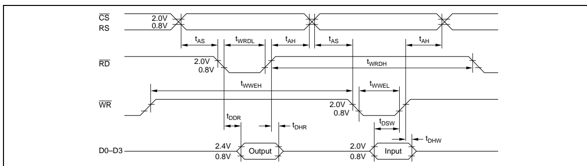
Figure 40 MPU Interface
