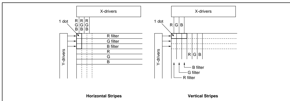
Figure 6 Stripe Modes in 8-Color Display
