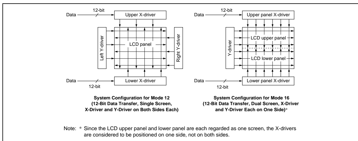
Figure 7 System Configurations by Mode (cont)
