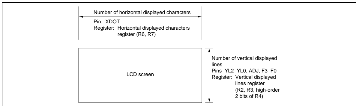
Figure 4 Relationship between LCD Screen and Pins and Internal Registers
