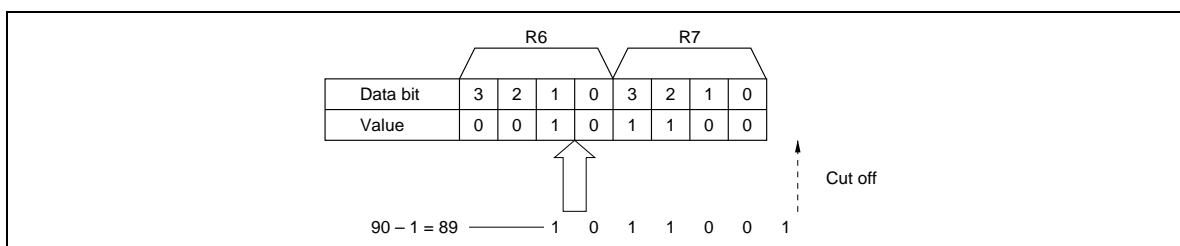
Figure 24 How to Write the Number of Horizontal Displayed Characters
