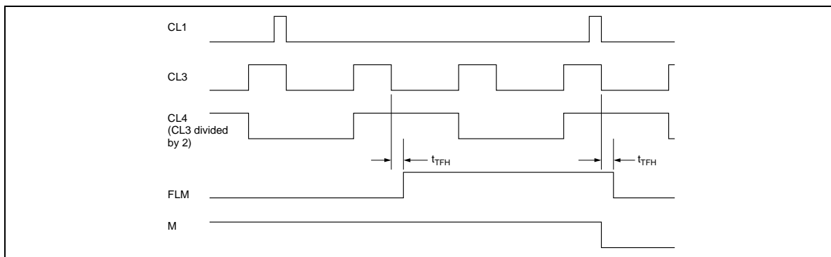
Figure 39 CL1, CL3, CL4, FLM, and M in Horizontal Stripe Modes (Expanded Detail of Figure 38)
