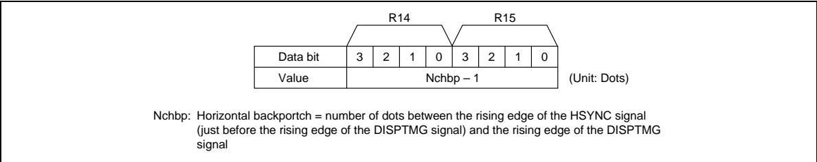
Figure 29 Horizontal Backporch Register
