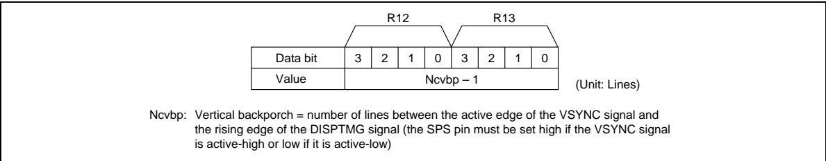
Figure 28 Vertical Backporch Register
