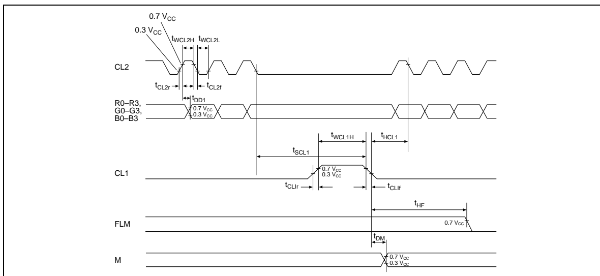
Figure 36 TN-Type LCD Driver Interface
