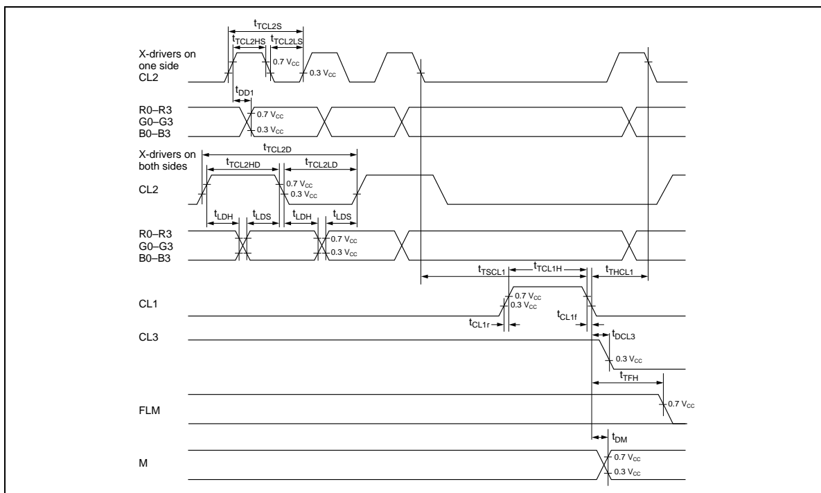
Figure 38 TFT-Type LCD Driver Interface
