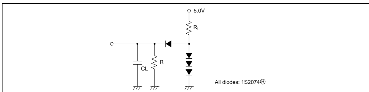
Figure 44 TTL Load Circuit
