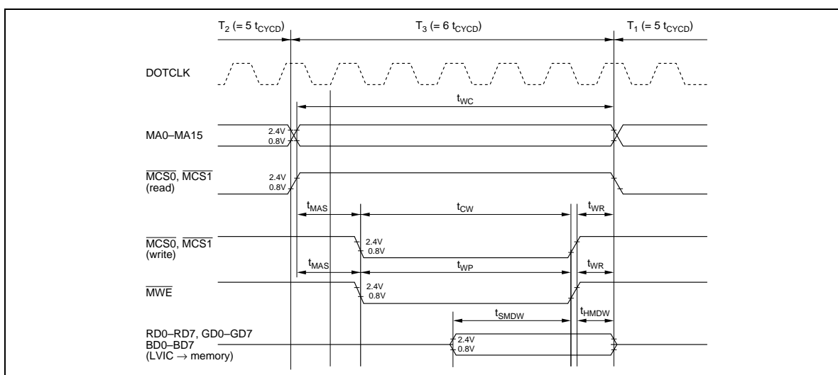
Figure 35 Buffer Memory Interface (RAM Write Timing)
