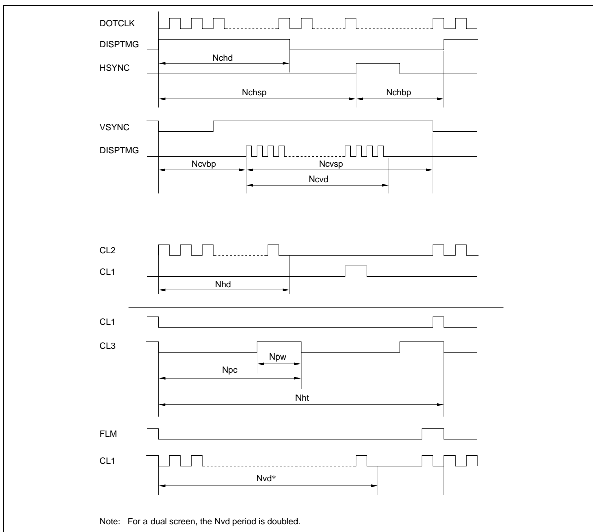
Figure 32 Symbol Definitions
