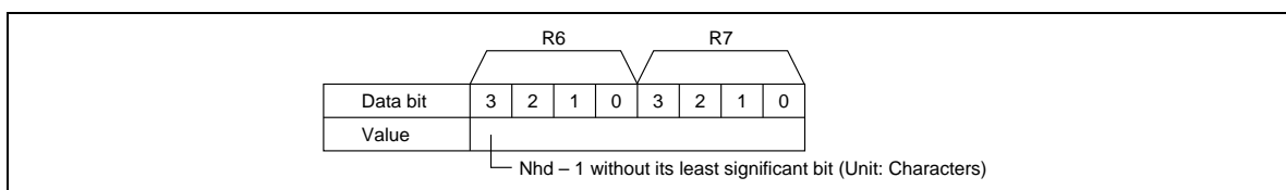
Figure 23 Horizontal Displayed Characters Register
