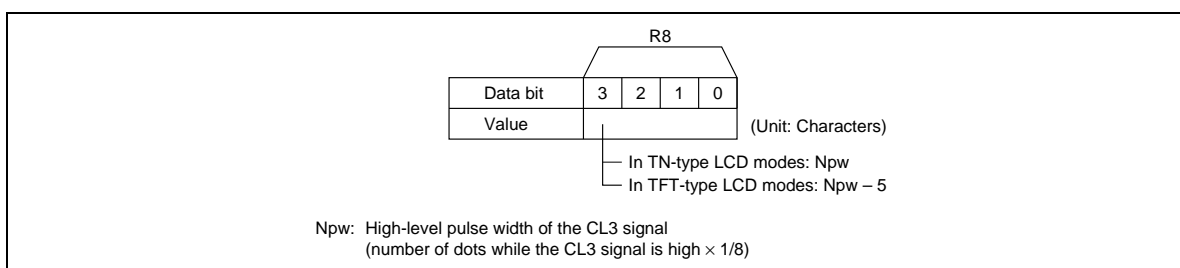
Figure 25 CL3 Pulse Width Register
