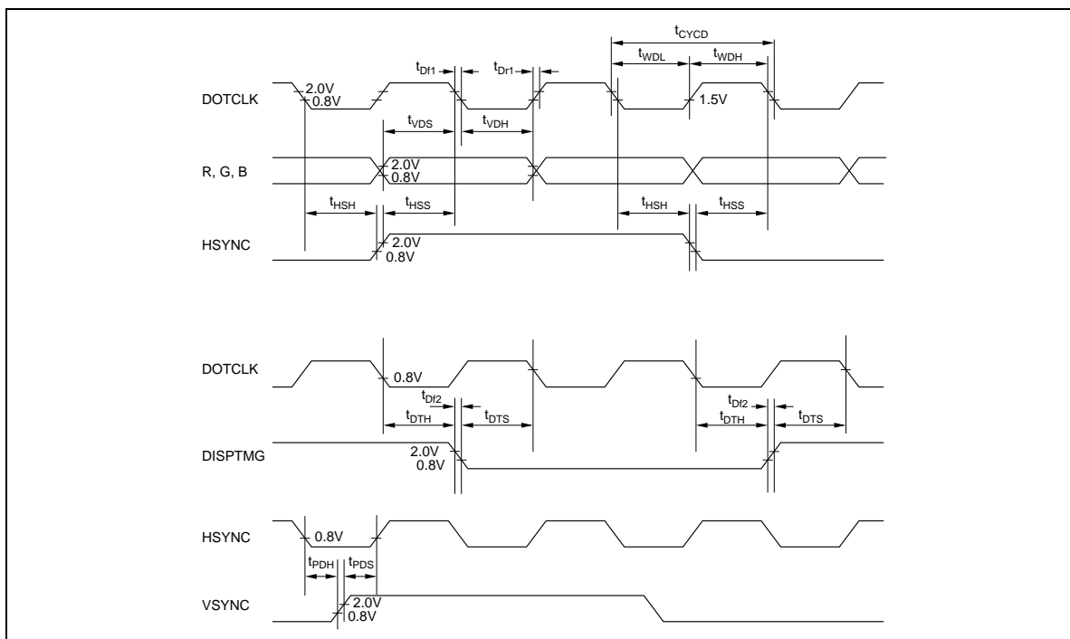
Figure 33 Video Signal Interface
