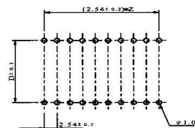
P.C.D. HOLE PATTERNS FOR SOCKETS
