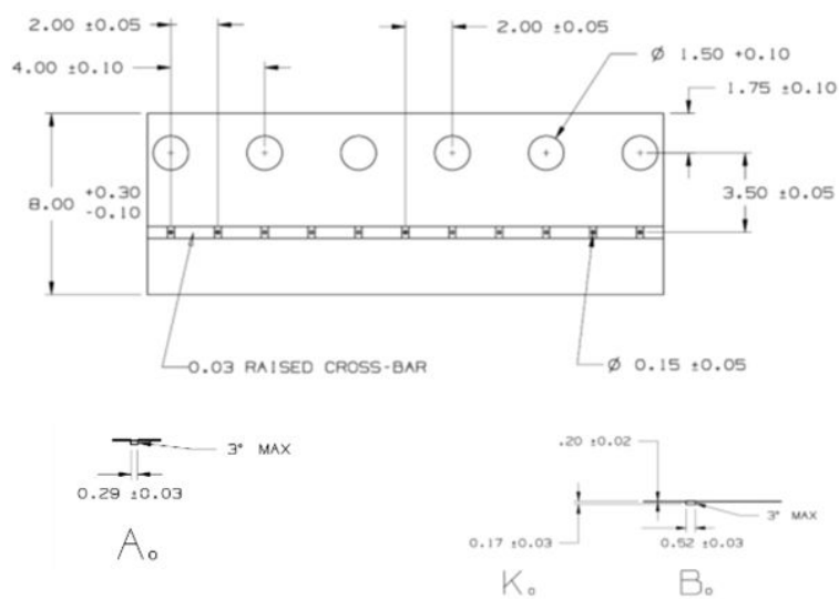
Figure 10. Tape and reel mechanical data
