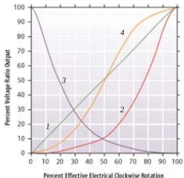
Figure 1: Popular Tapers
