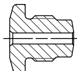
124451 DRIVING ANVIL -04
