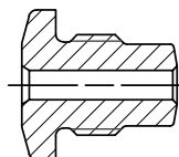
124450 DRIVING ANVIL -05
