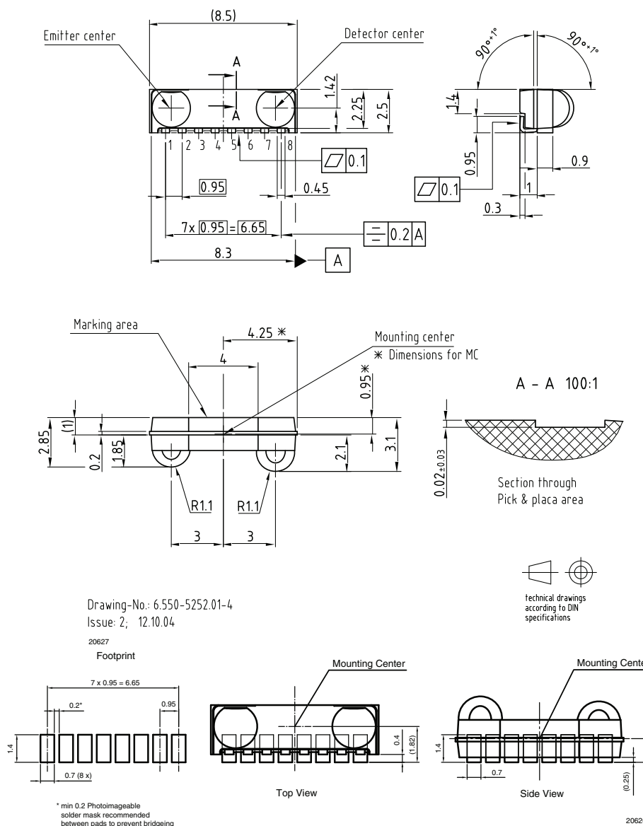
Fig. 8 - Package Drawing
