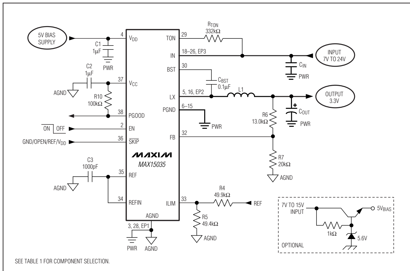
Figure 6. High Output-Voltage Application Using a Feedback Divider
