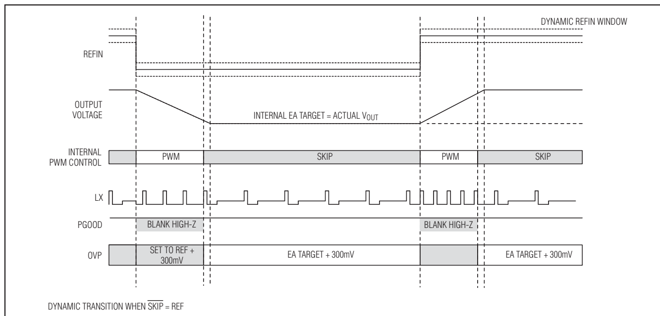
Figure 5. Dynamic Transition when \overline{\text{SKIP}} = \text{REF}
