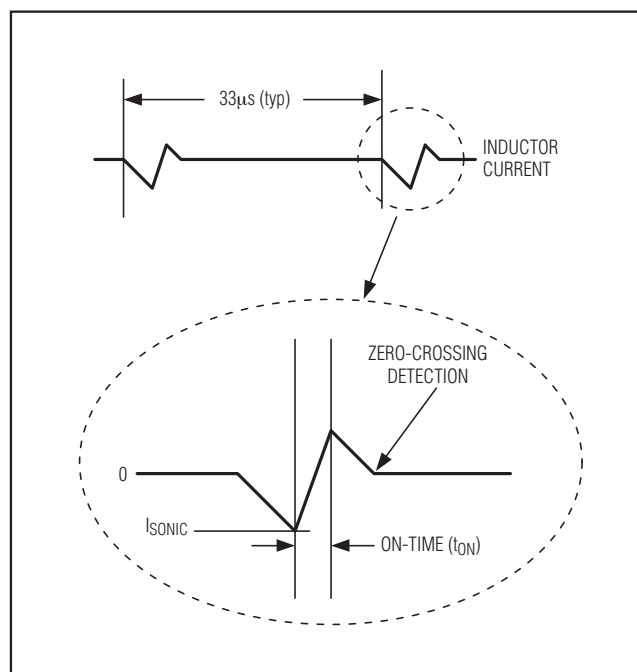
Figure 3. Ultrasonic Waveform
