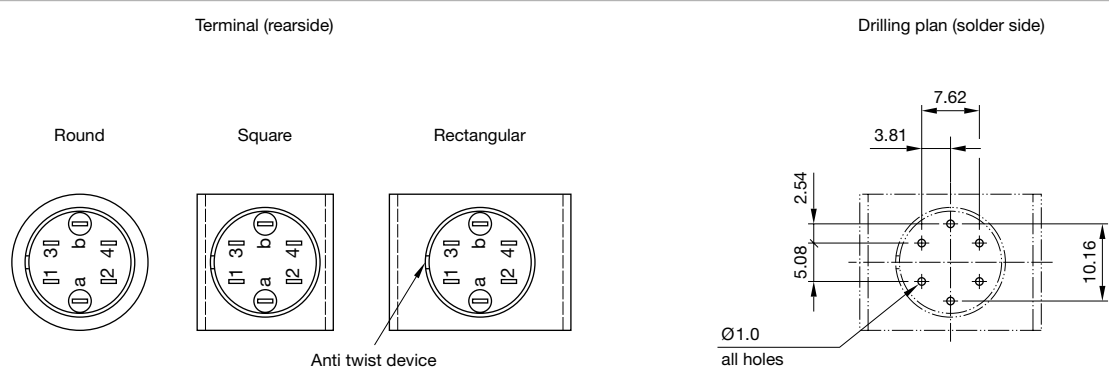
Component layout 3
