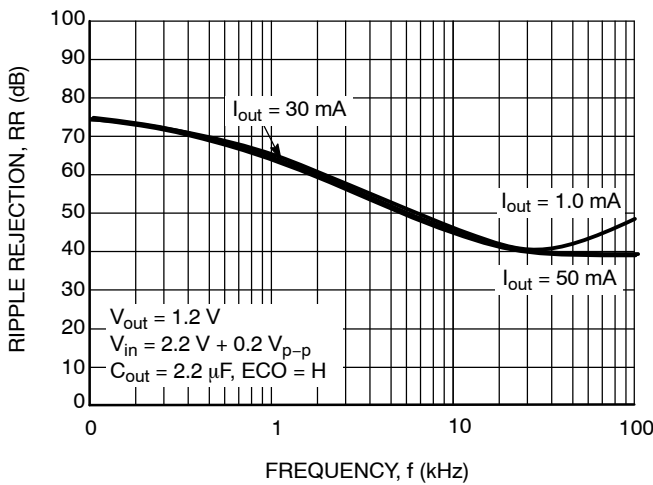
Figure 26. Ripple Rejection vs. Frequency
