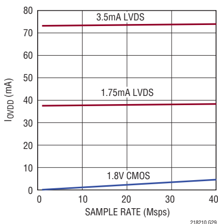
LTC2181: I_{OVDD} vs Sample Rate, 5MHz, -1dBFS, Sine Wave Input on Each Channel
