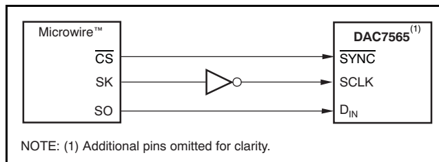
Figure 102. DAC7565 to Microwire Interface
