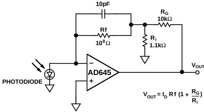
Figure 34. A Photodiode Preamplifier Employing a "T" Network for Added Gain
