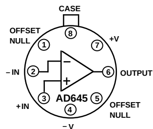
TO-99 (H) Package
