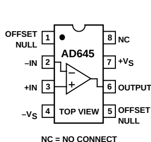
8-Pin Plastic Mini-DIP (N) Package
