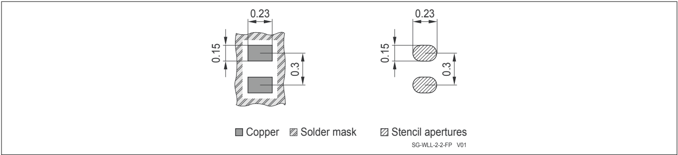
Figure 8 WLL-2-2 footprint (dimension in mm), recommendation for Printed Circuit Board assembly see [2]
