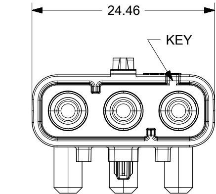
P/N 2018431030 KEY A
