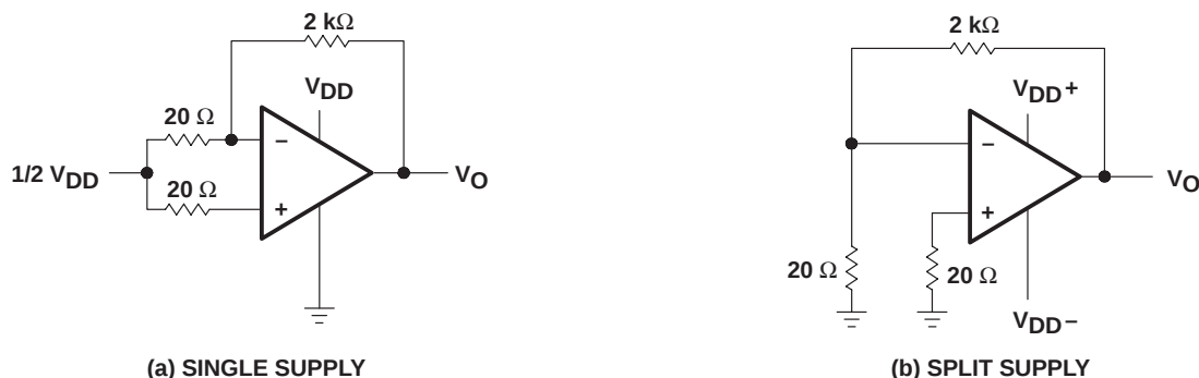
Figure 2. Noise-Test Circuit
