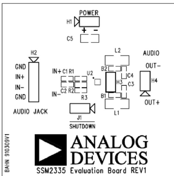
Figure 6. Top Silkscreen
