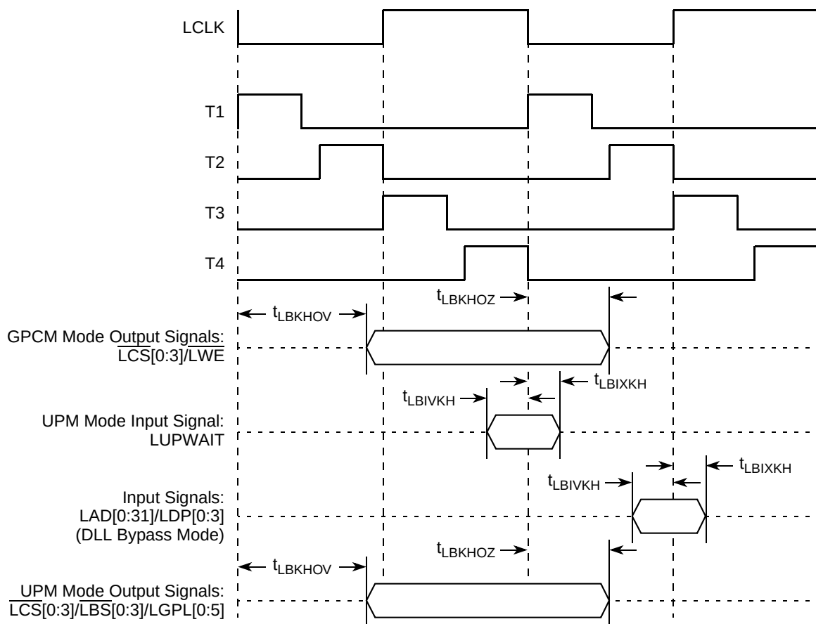
Figure 27. Local Bus Signals, GPCM/UPM Signals for \text{LCRR}[\text{CLKDIV}] = 4 (DLL Bypass Mode)
