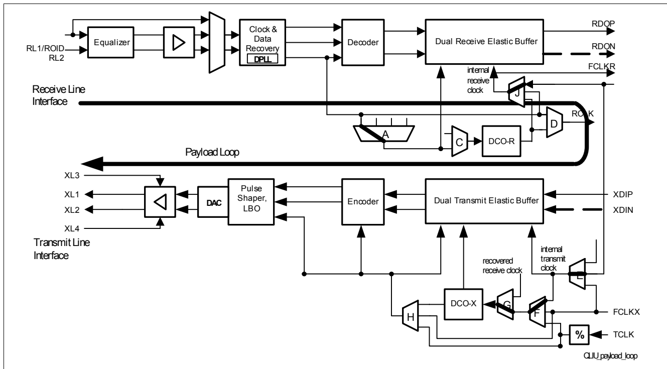
Figure 45 Payload Loop
