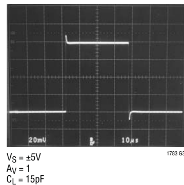
Small-Signal Response
