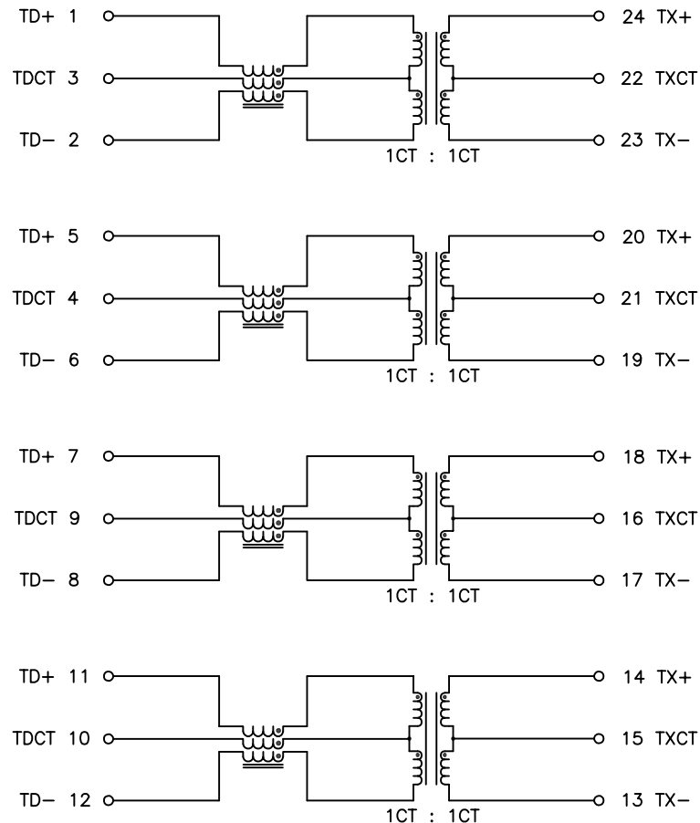
SCHEMATIC
