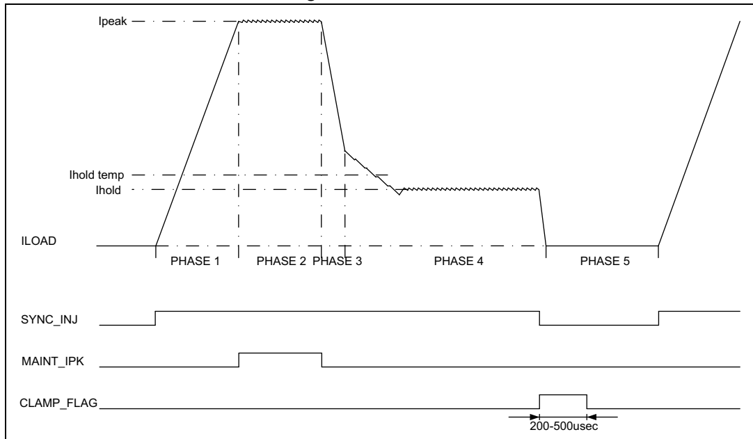
Figure 2. Waveforms
