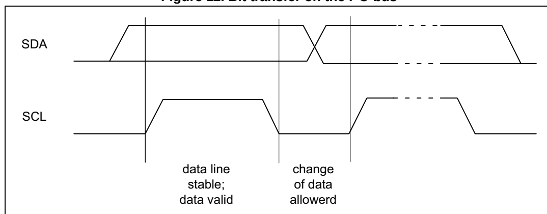
Figure 11. Bit transfer on the I 2 C-bus
