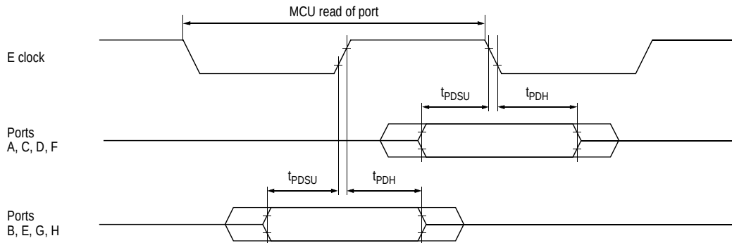
Figure 12-7. Port read timing diagram
