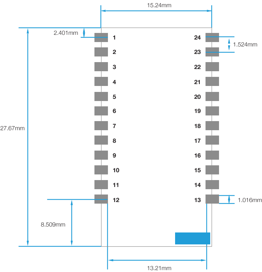
Module dimension and suggested landing pattern (shown dimensions not to scale)
