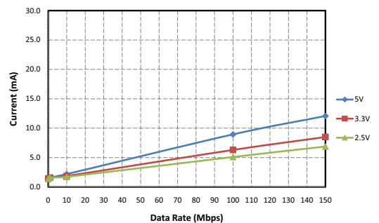
Figure 13. Si8620 Typical V_{DD2} Supply Current vs. Data Rate 5, 3.3, and 2.70 V Operation (15 pF Load)
