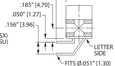
RIGHT ANGLE, DIP SOLDER (RA, SA)
