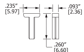
PLM-K2 KEY IN CONTACT (ORDER SEPARATELY)
