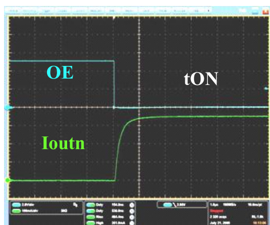
Figure 17: t_{ON}
