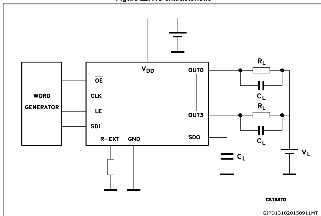
Figure 12: AC characteristic
