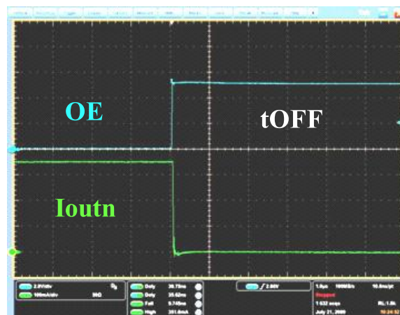
Figure 18: t_{OFF}
