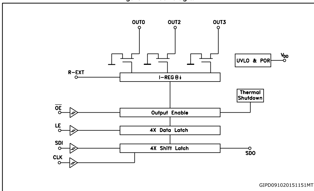
Figure 1: Block diagram
