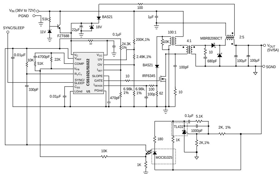
36-72V to 5V, 5A DC-DC Convertor
