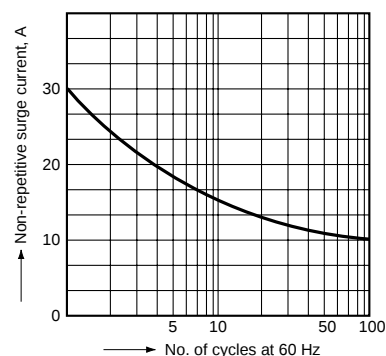
2-1. Non-repetitive surge current vs. time characteristics (OAC)
