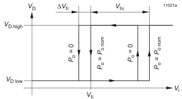
Fig. 22 Definition of V_{ti} , \Delta V_{ti} , and V_h (JFET output)
